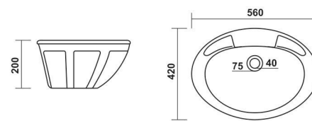
102-OVEL TOP COUNTER
