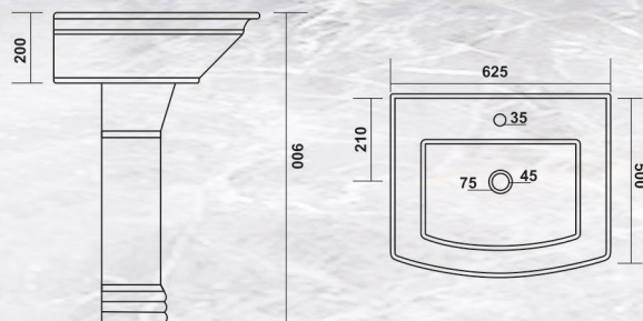
SILVER SET WB 8005 - PED 9004 L 625 W 500 H 900mm
